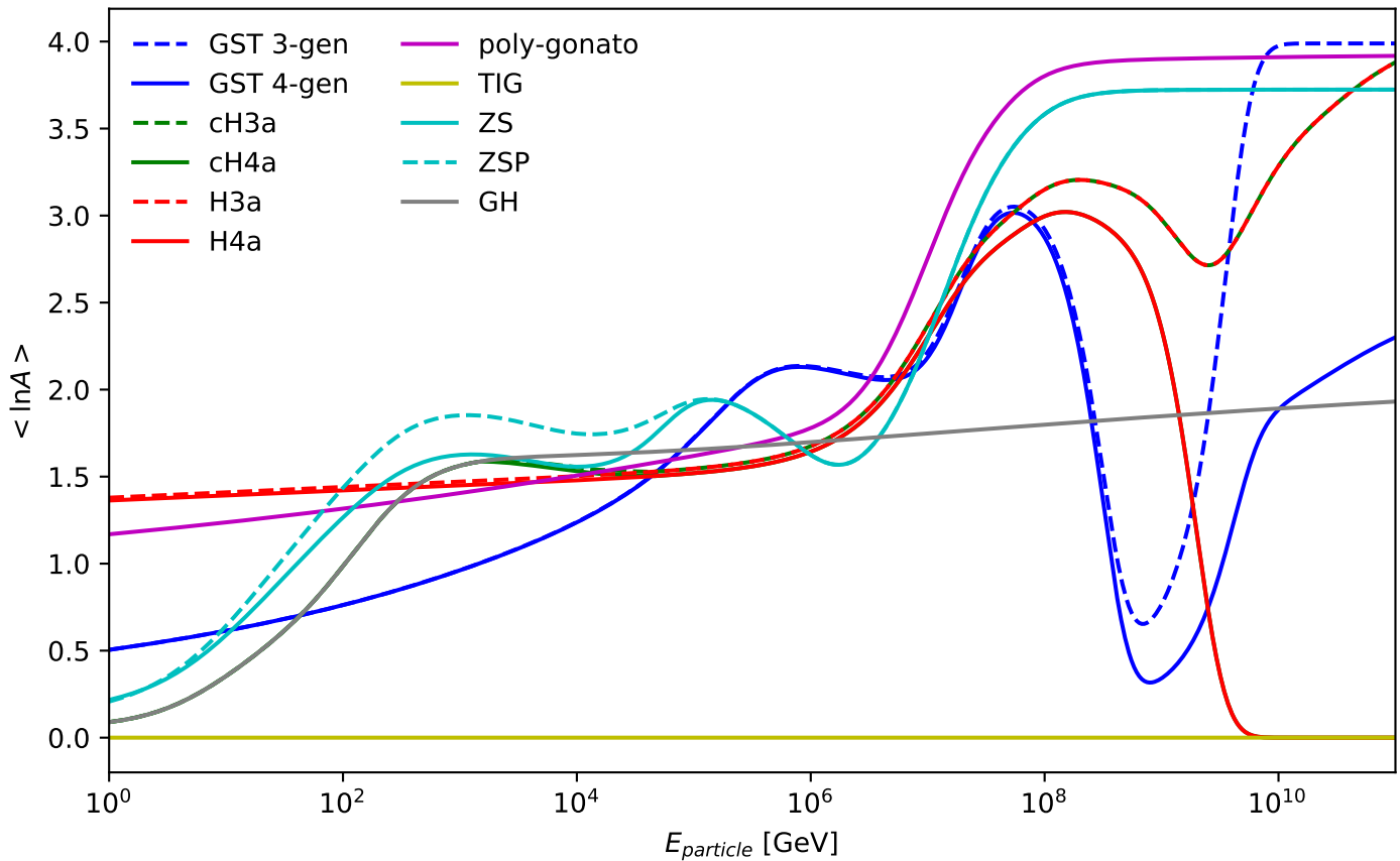
Mean log mass \langle \ln A \rangle .
