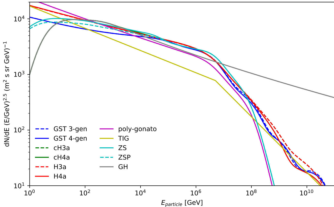
Cosmic ray particle flux (all-nuclei).
