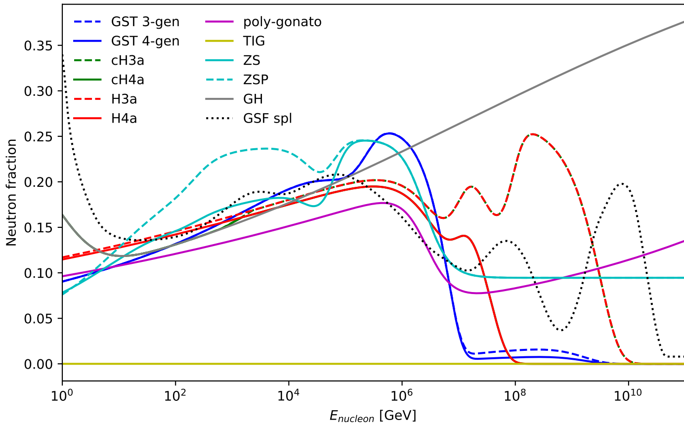
Fraction of neutrons relative to protons.
