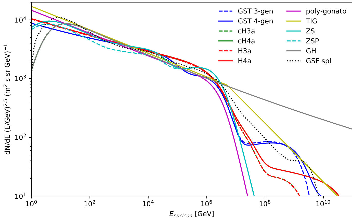
Cosmic ray nucleon flux (proton + neutron)
